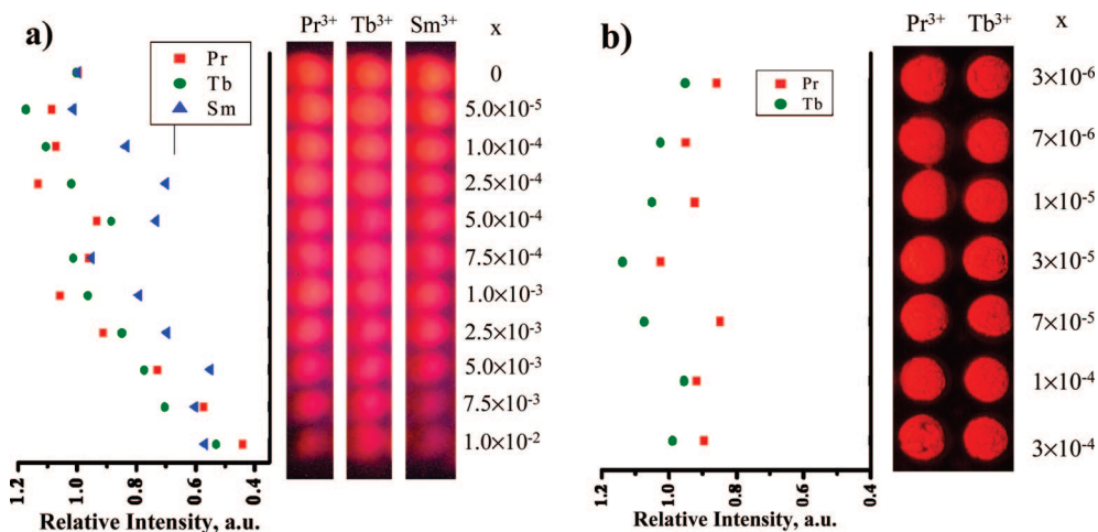
Figure 2. Composition maps, VUV photoluminescence photographs, and the calibrated photoluminescent intensities as the functions of composition of the (a) primary and (b) secondary combinatorial libraries at 147 nm excitation: red square, Pr 3+ co-doped (Y 0.65 Gd 0.35 )BO 3 :Eu 3+ 0.05 ; green circle, Tb 3+ co-doped (Y 0.65 Gd 0.35 )BO 3 :Eu 3+ 0.05 ; blue triangle, Sm 3+ co-doped (Y 0.65 Gd 0.35 )BO 3 :Eu 3+ 0.05 .
